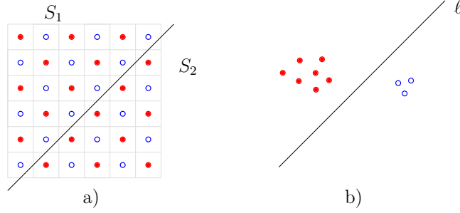
Figure 2: a) A bicolored grid with coarseness 3. b) The coarseness is not given by the separation line \ell .
